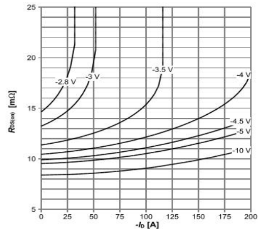
Figure 4: Rdson- Drain Current
