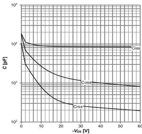
Figure 3: Capacitance
