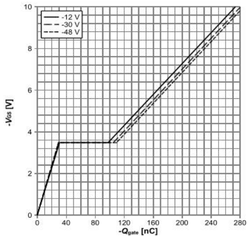
Figure 5: Gate-Charge Characteristics
