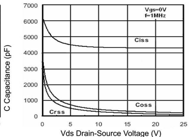
Figure 4. Capacitance Characteristics
