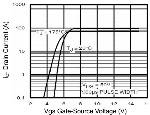
Figure 3. Transfer Characteristics
