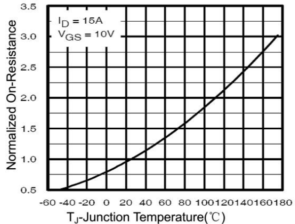
Figure 2. On-Resistance Variation with Temperature
